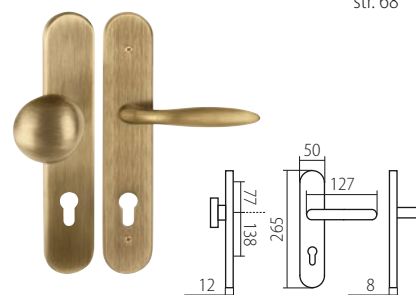
COLUMBUS BLOCK HR H 2094 KS DEF
