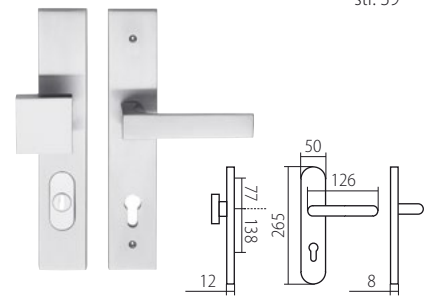
DAVID HTSI 4500 ARIA DEF
