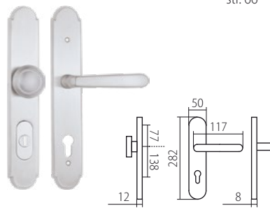
DAVID HTSI 4500 INNER DEF
