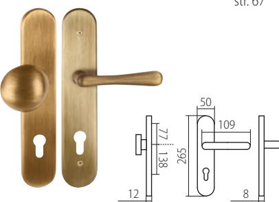
COLUMBUS ALFA HR H 2094 KS DEF
