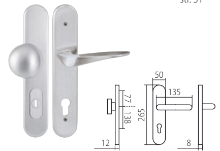
DAVID HTSI 4500 NICOL DEF
